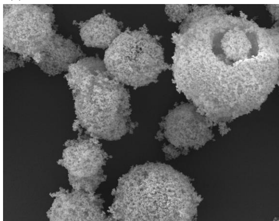
Figure 1: MOFs (HKUST-1) beads of 80 µm in diameter prepared by spray-drying process
